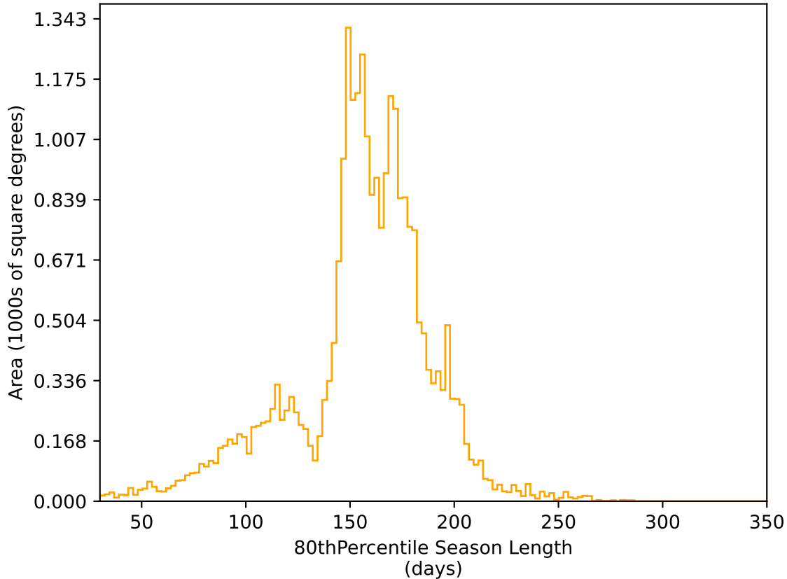
too_elab_heavy_r128_d3_ugrizy_v3.4_10yrs All sky r band: 80thPercentile Season Length
