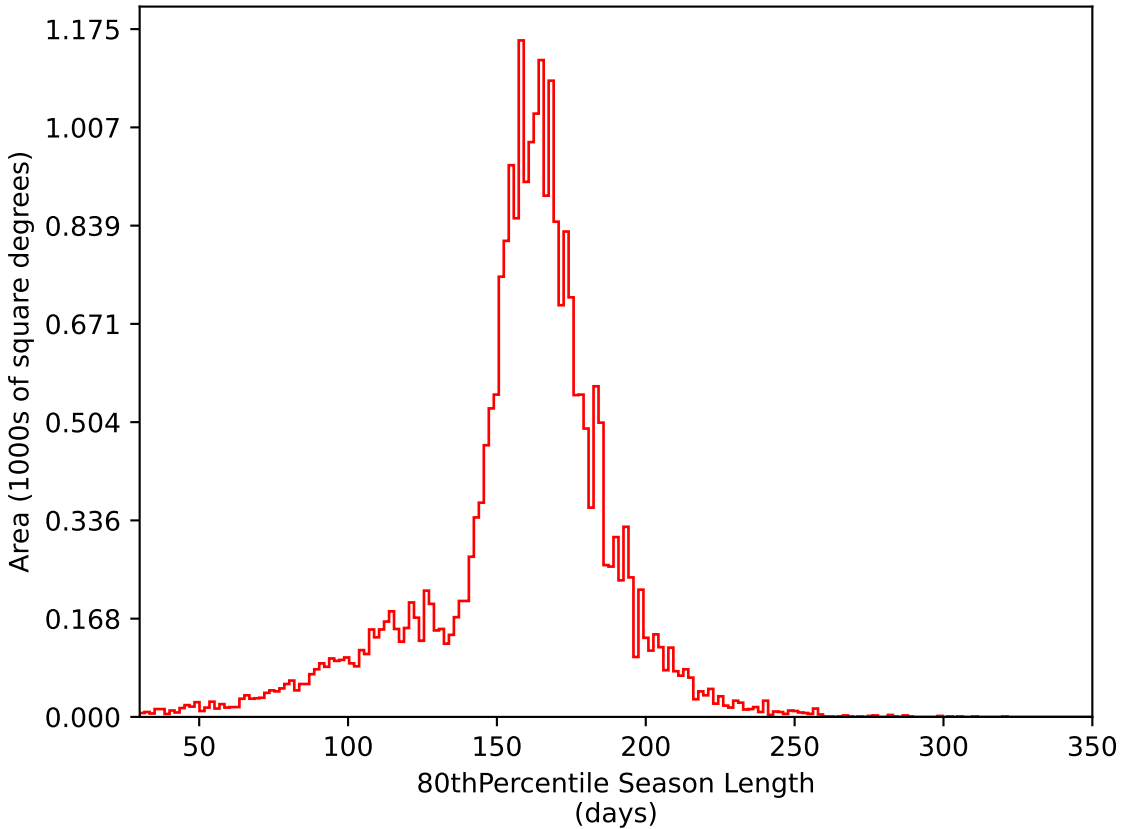
too_elab_heavy_r128_d3_ugrizy_v3.4_10yrs All sky i band: 80thPercentile Season Length
