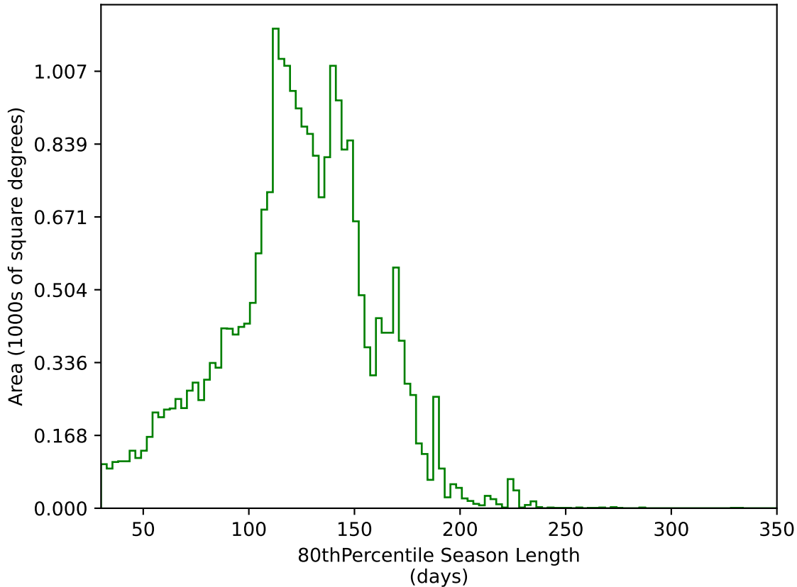
too_elab_heavy_r128_d3_ugrizy_v3.4_10yrs All sky g band: 80thPercentile Season Length
