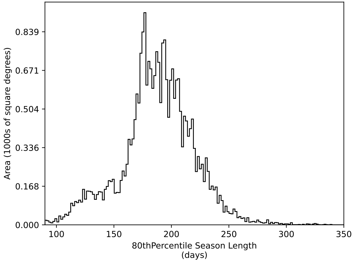
too_elab_heavy_r128_d3_ugrizy_v3.4_10yrs All sky all bands: 80thPercentile Season Length
