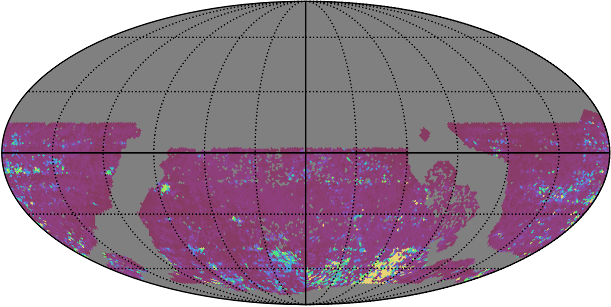
too_elab_heavy_r128_d3_ugrizy_v3.4_10yrs WFD z band: 75th Percentile Intranight Timespan
