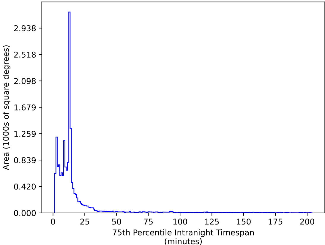
too_elab_heavy_r128_d3_ugrizy_v3.4_10yrs WFD z band: 75th Percentile Intranight Timespan
