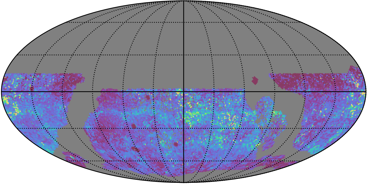
too_elab_heavy_r128_d3_ugrizy_v3.4_10yrs WFD y band: 75th Percentile Intranight Timespan
