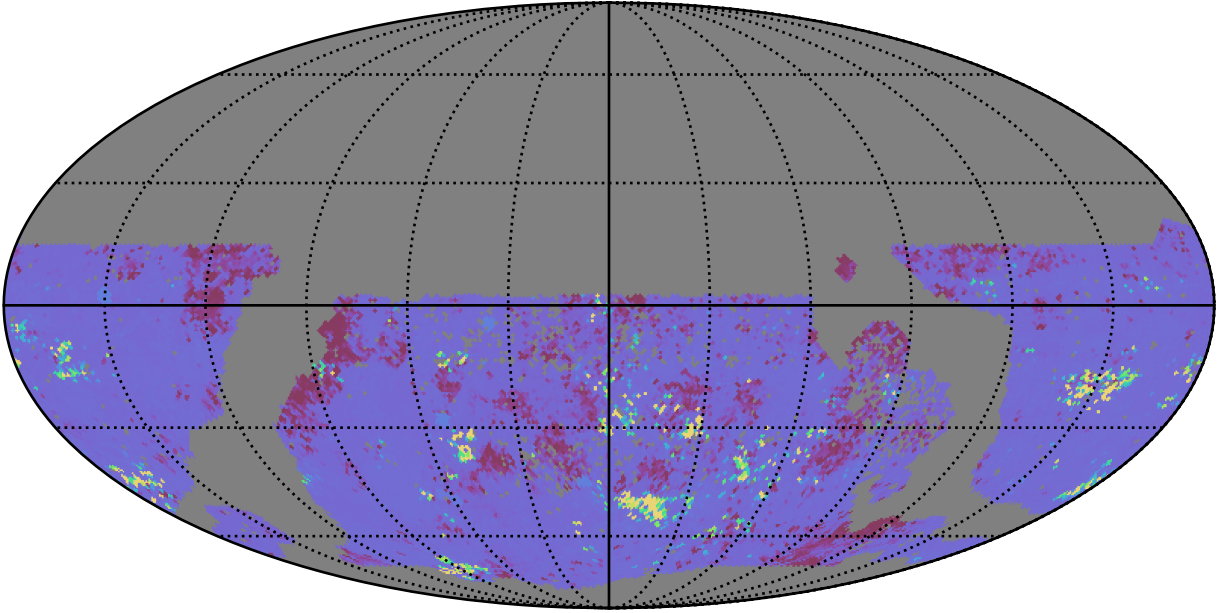
too_elab_heavy_r128_d3_ugrizy_v3.4_10yrs WFD ug bands: 75th Percentile Intranight Timespan
