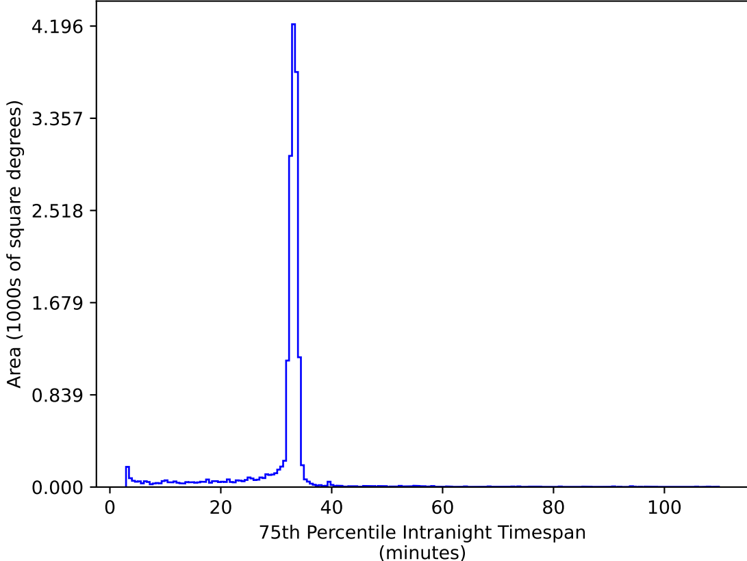
too_elab_heavy_r128_d3_ugrizy_v3.4_10yrs WFD ug bands: 75th Percentile Intranight Timespan
