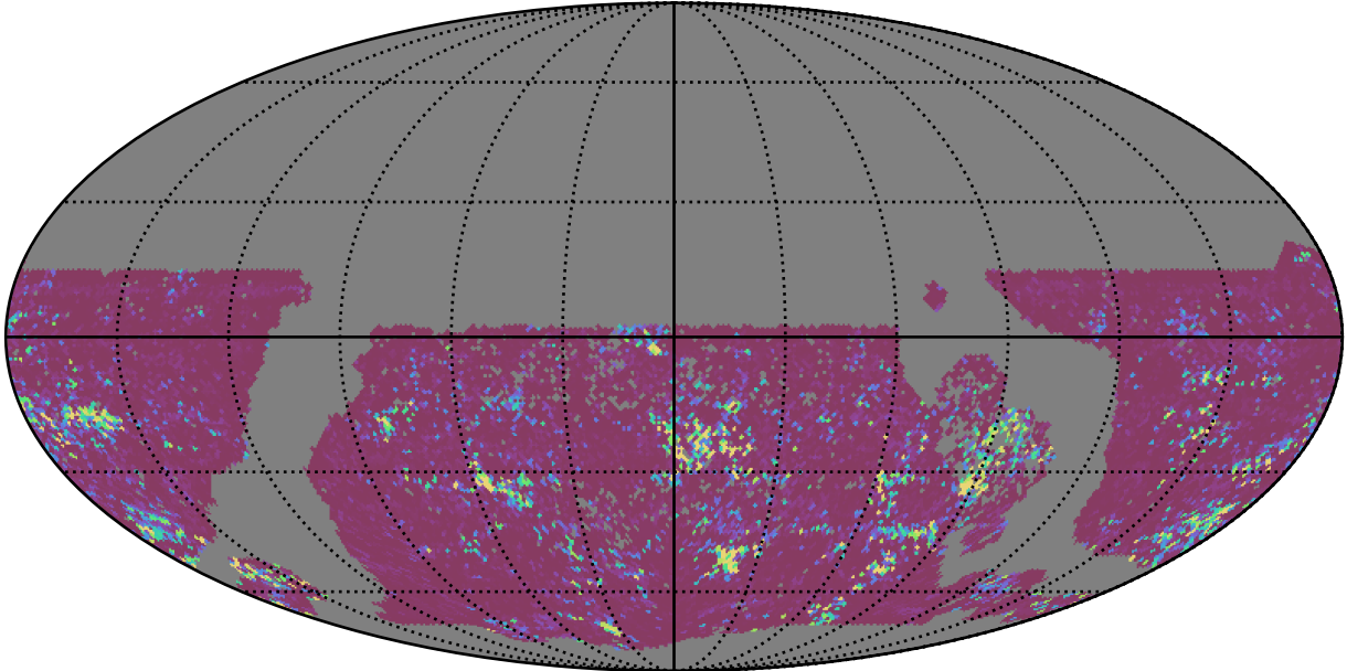
too_elab_heavy_r128_d3_ugrizy_v3.4_10yrs WFD u band: 75th Percentile Intranight Timespan
