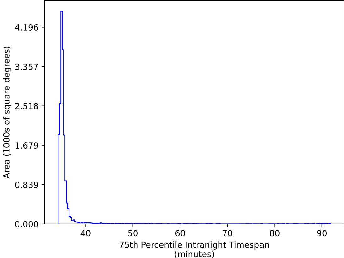
too_elab_heavy_r128_d3_ugrizy_v3.4_10yrs WFD ri bands: 75th Percentile Intranight Timespan
