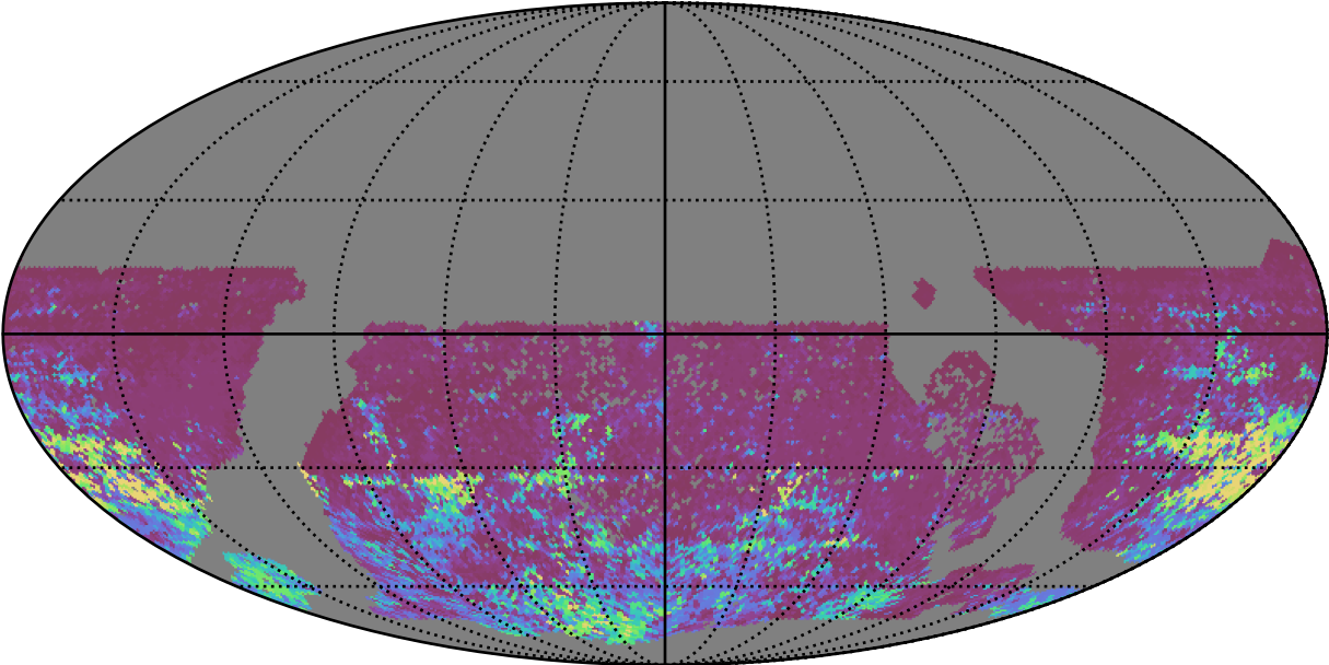
too_elab_heavy_r128_d3_ugrizy_v3.4_10yrs WFD r band: 75th Percentile Intranight Timespan
