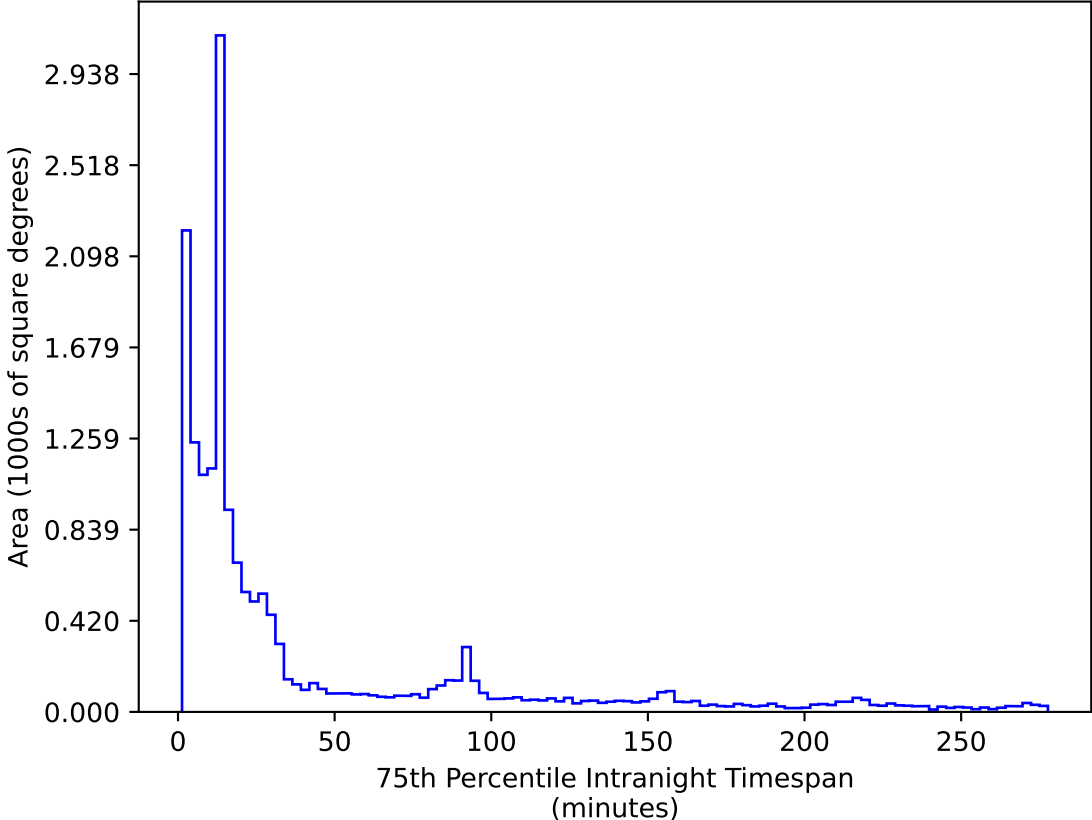
too_elab_heavy_r128_d3_ugrizy_v3.4_10yrs WFD r band: 75th Percentile Intranight Timespan
