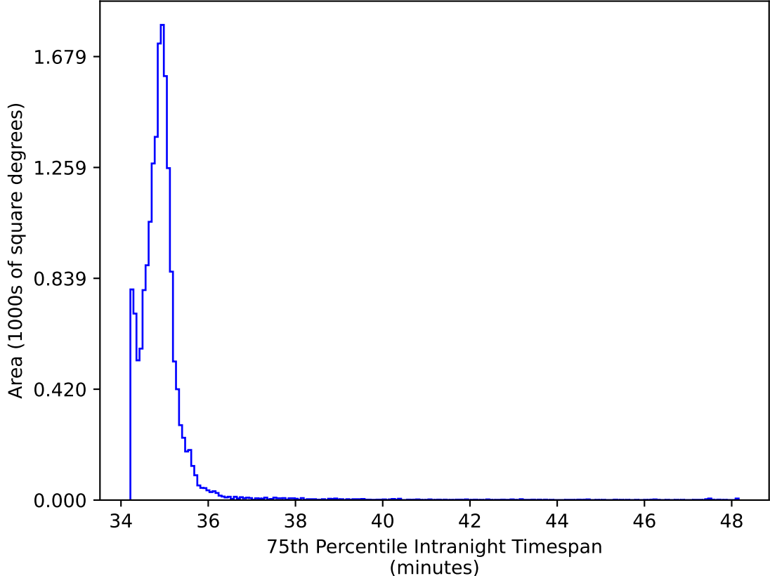
too_elab_heavy_r128_d3_ugrizy_v3.4_10yrs WFD iz bands: 75th Percentile Intranight Timespan
