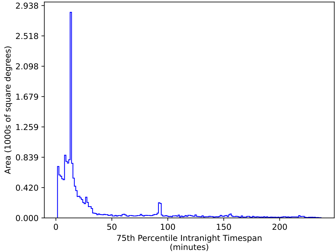
too_elab_heavy_r128_d3_ugrizy_v3.4_10yrs WFD i band: 75th Percentile Intranight Timespan
