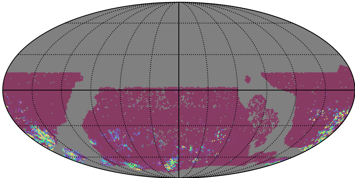
too_elab_heavy_r128_d3_ugrizy_v3.4_10yrs WFD gr bands: 75th Percentile Intranight Timespan
