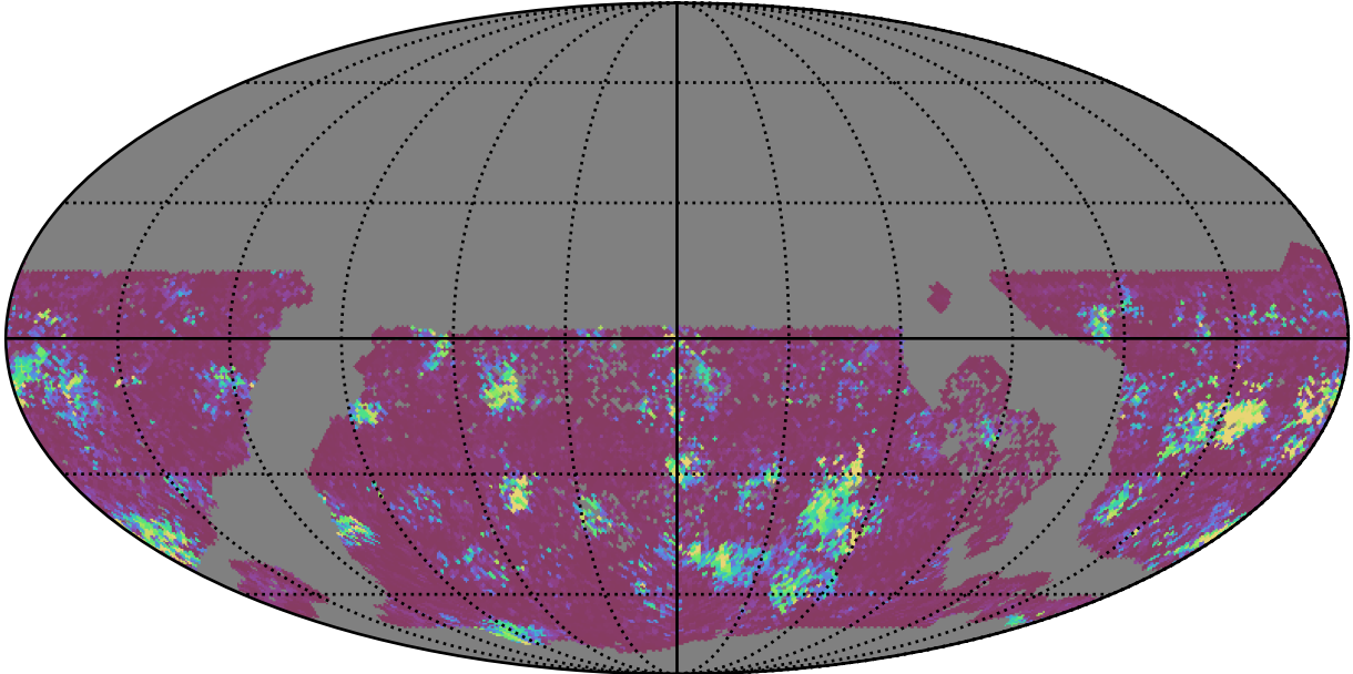
too_elab_heavy_r128_d3_ugrizy_v3.4_10yrs WFD g band: 75th Percentile Intranight Timespan
