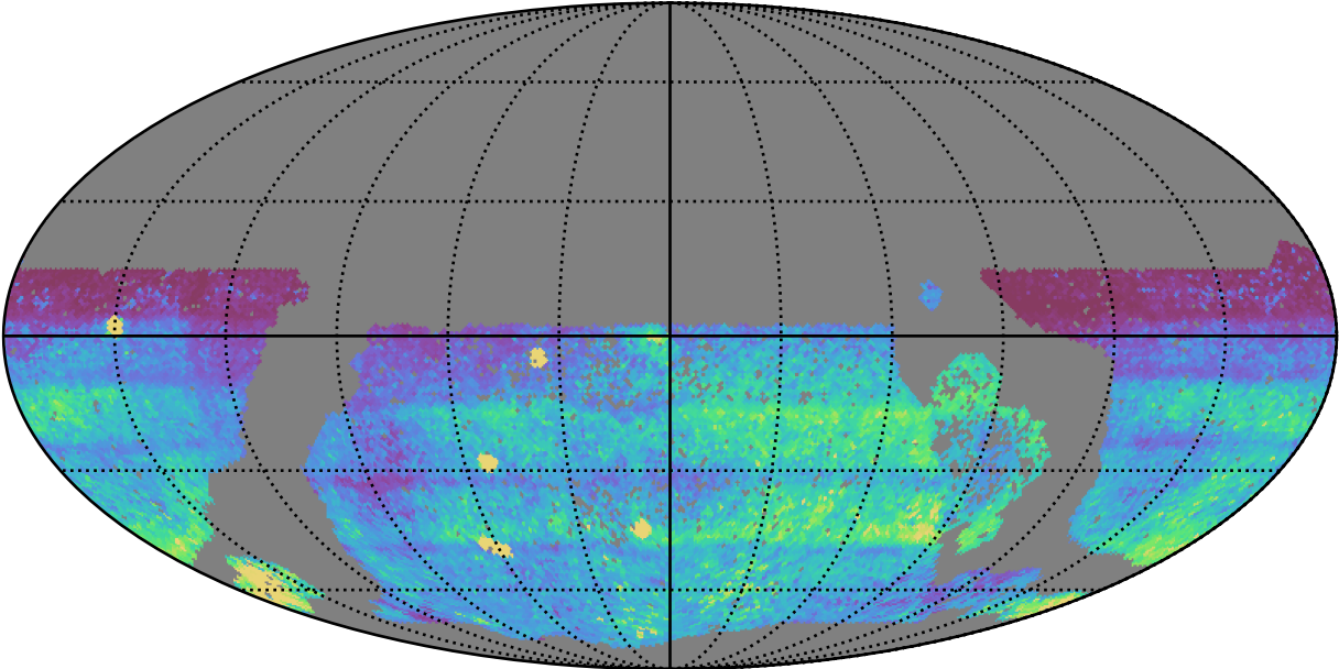
too_elab_heavy_r128_d3_ugrizy_v3.4_10yrs WFD all bands: 75th Percentile Intranight Timespan
