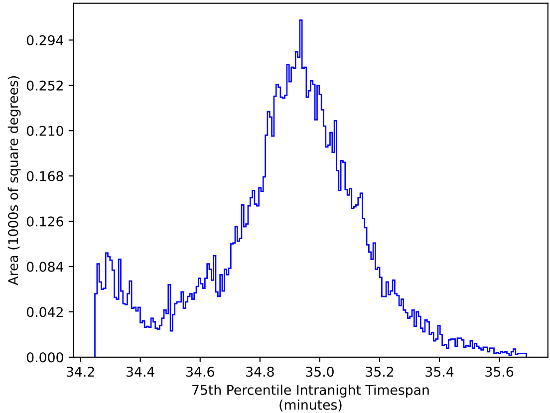
too_elab_heavy_r128_d3_ugrizy_v3.4_10yrs WFD all bands: 75th Percentile Intranight Timespan
