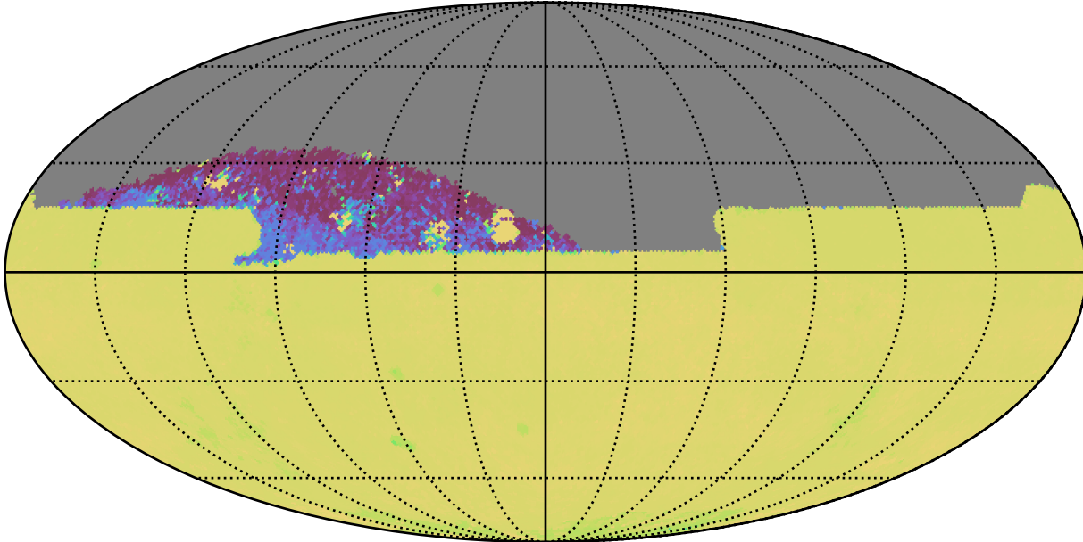
too_elab_heavy_r128_d3_ugrizy_v3.4_10yrs All sky zy bands: 75th Percentile Intranight Timespan
