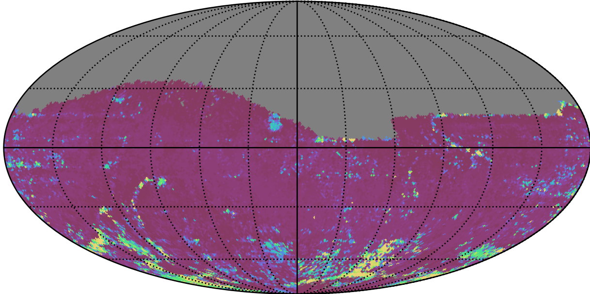
too_elab_heavy_r128_d3_ugrizy_v3.4_10yrs All sky z band: 75th Percentile Intranight Timespan
