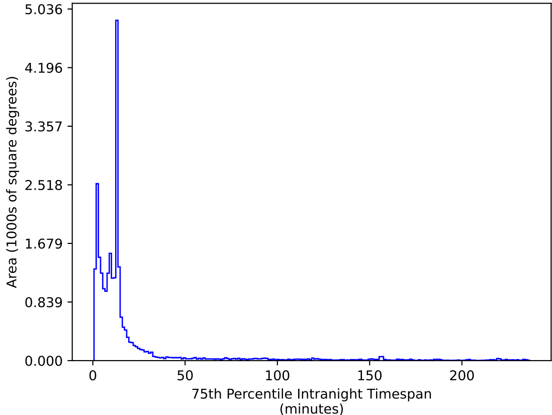
too_elab_heavy_r128_d3_ugrizy_v3.4_10yrs All sky z band: 75th Percentile Intranight Timespan
