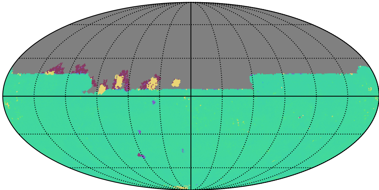
too_elab_heavy_r128_d3_ugrizy_v3.4_10yrs All sky y band: 75th Percentile Intranight Timespan
