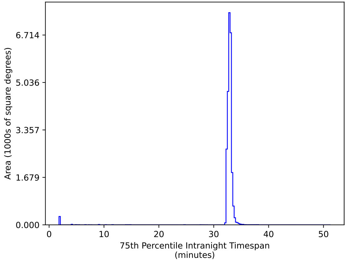
too_elab_heavy_r128_d3_ugrizy_v3.4_10yrs All sky y band: 75th Percentile Intranight Timespan
