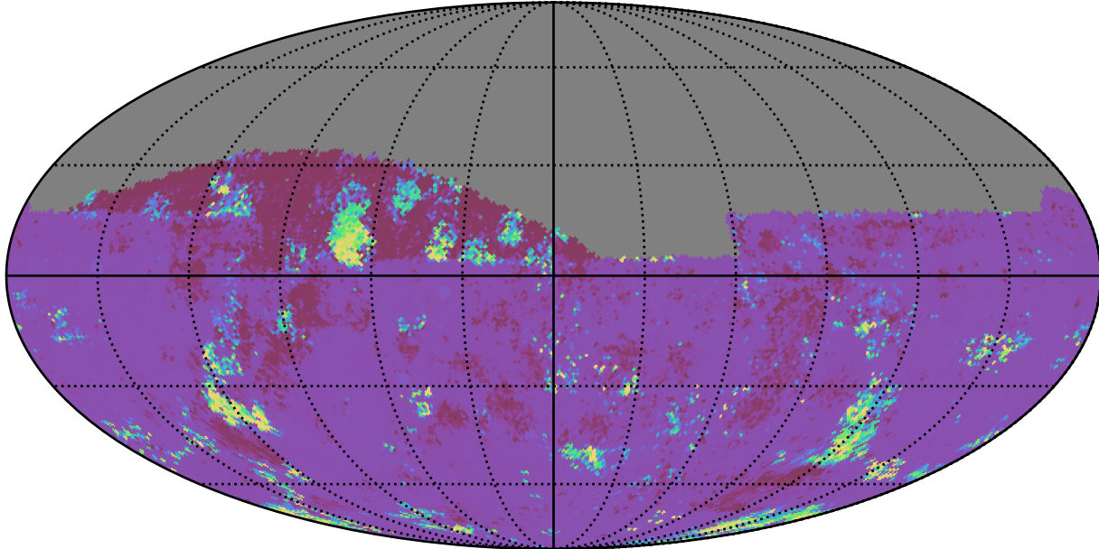
too_elab_heavy_r128_d3_ugrizy_v3.4_10yrs All sky ug bands: 75th Percentile Intranight Timespan
