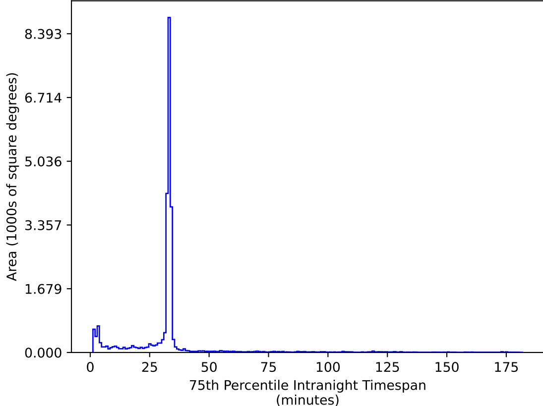
too_elab_heavy_r128_d3_ugrizy_v3.4_10yrs All sky ug bands: 75th Percentile Intranight Timespan
