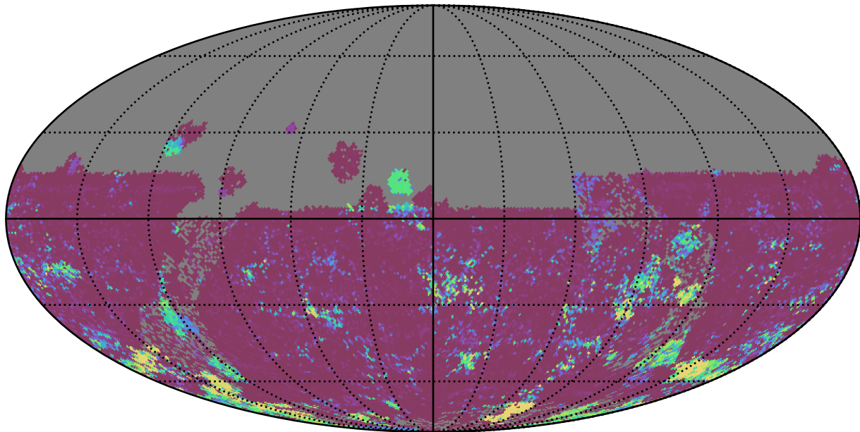
too_elab_heavy_r128_d3_ugrizy_v3.4_10yrs All sky u band: 75th Percentile Intranight Timespan
