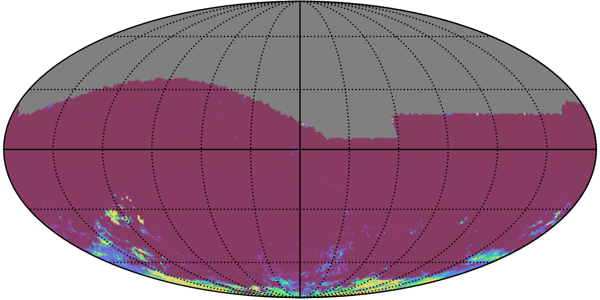
too_elab_heavy_r128_d3_ugrizy_v3.4_10yrs All sky ri bands: 75th Percentile Intranight Timespan
