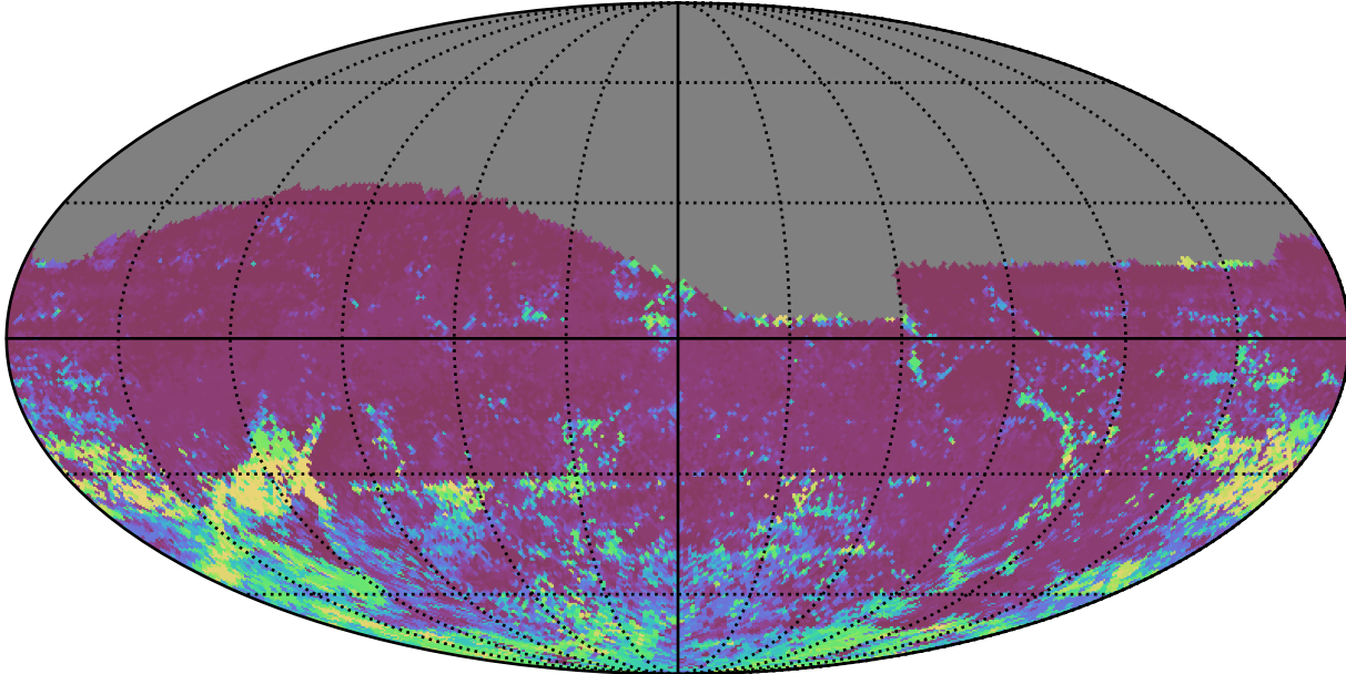
too_elab_heavy_r128_d3_ugrizy_v3.4_10yrs All sky r band: 75th Percentile Intranight Timespan
