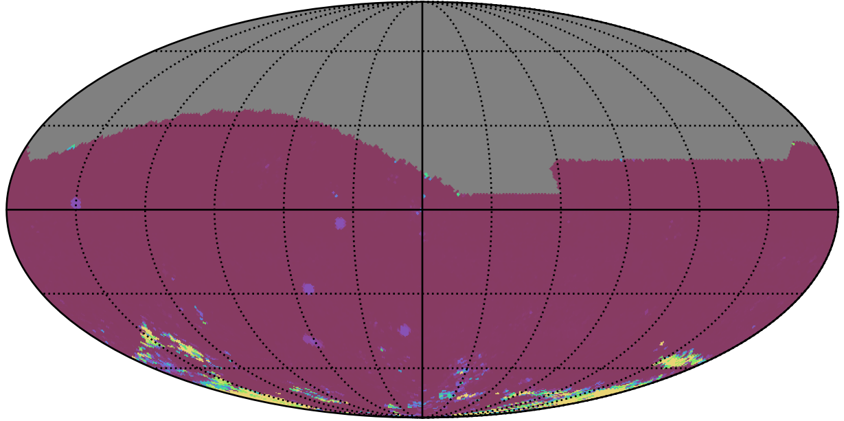
too_elab_heavy_r128_d3_ugrizy_v3.4_10yrs All sky iz bands: 75th Percentile Intranight Timespan
