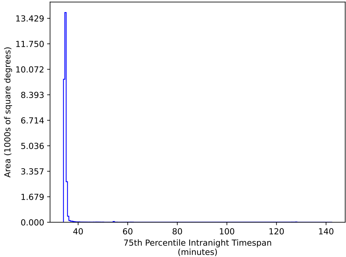
too_elab_heavy_r128_d3_ugrizy_v3.4_10yrs All sky iz bands: 75th Percentile Intranight Timespan
