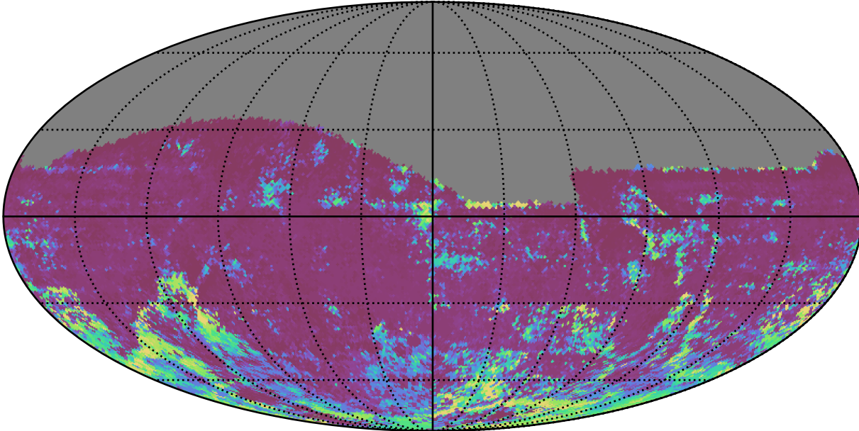
too_elab_heavy_r128_d3_ugrizy_v3.4_10yrs All sky i band: 75th Percentile Intranight Timespan
