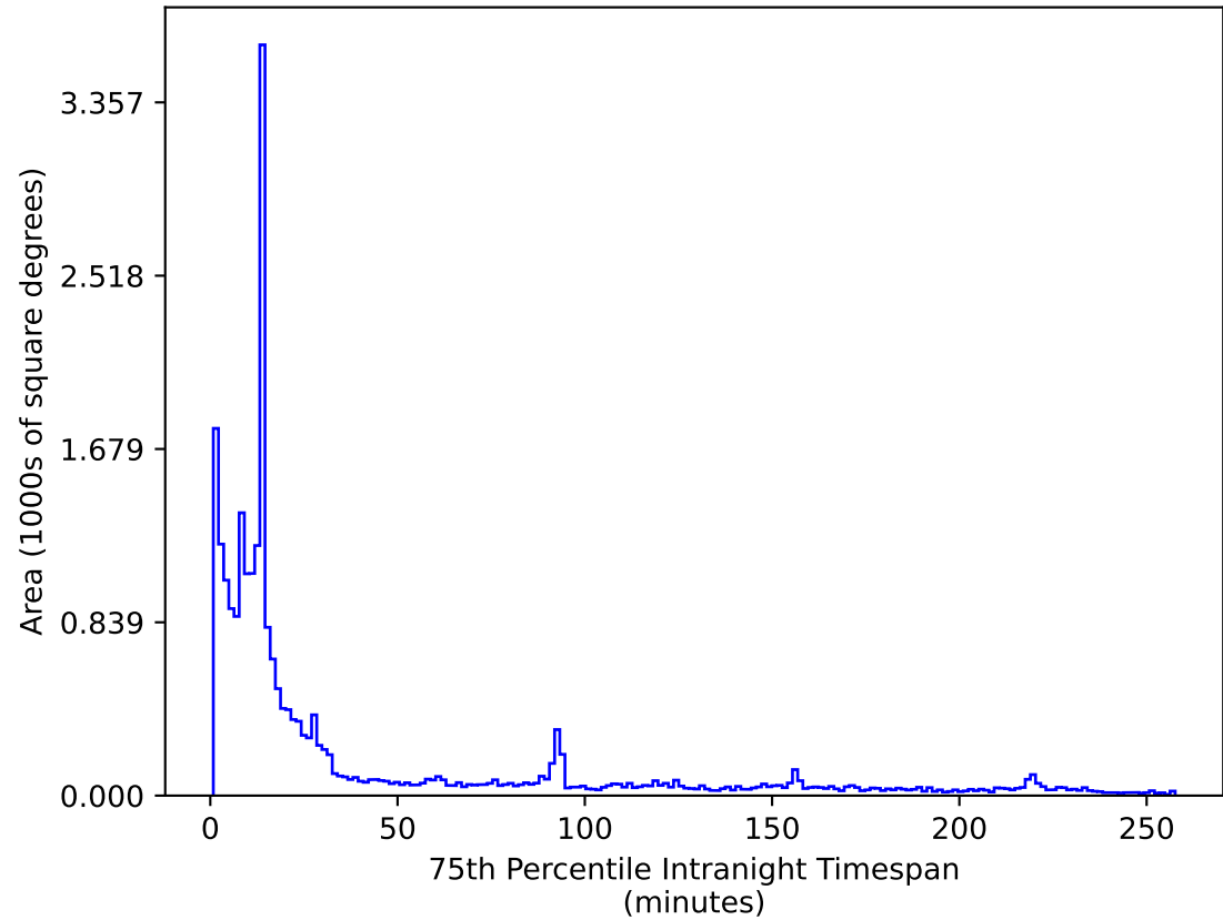
too_elab_heavy_r128_d3_ugrizy_v3.4_10yrs All sky i band: 75th Percentile Intranight Timespan
