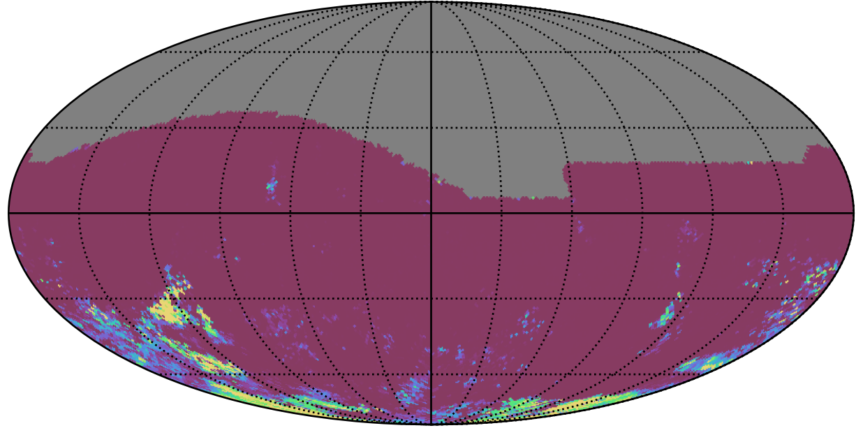
too_elab_heavy_r128_d3_ugrizy_v3.4_10yrs All sky gr bands: 75th Percentile Intranight Timespan
