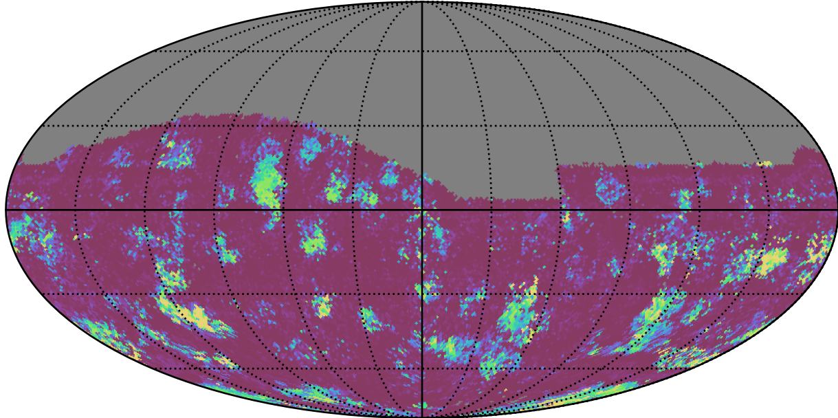
too_elab_heavy_r128_d3_ugrizy_v3.4_10yrs All sky g band: 75th Percentile Intranight Timespan
