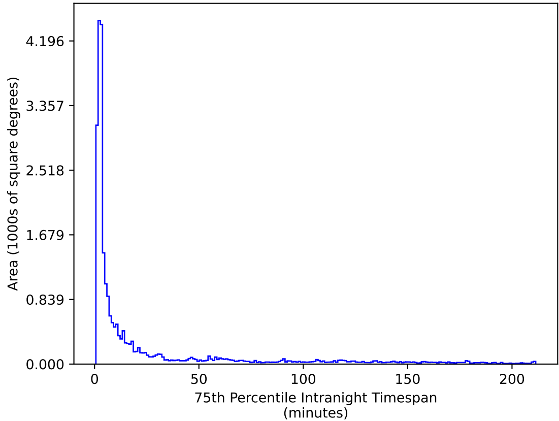
too_elab_heavy_r128_d3_ugrizy_v3.4_10yrs All sky g band: 75th Percentile Intranight Timespan
