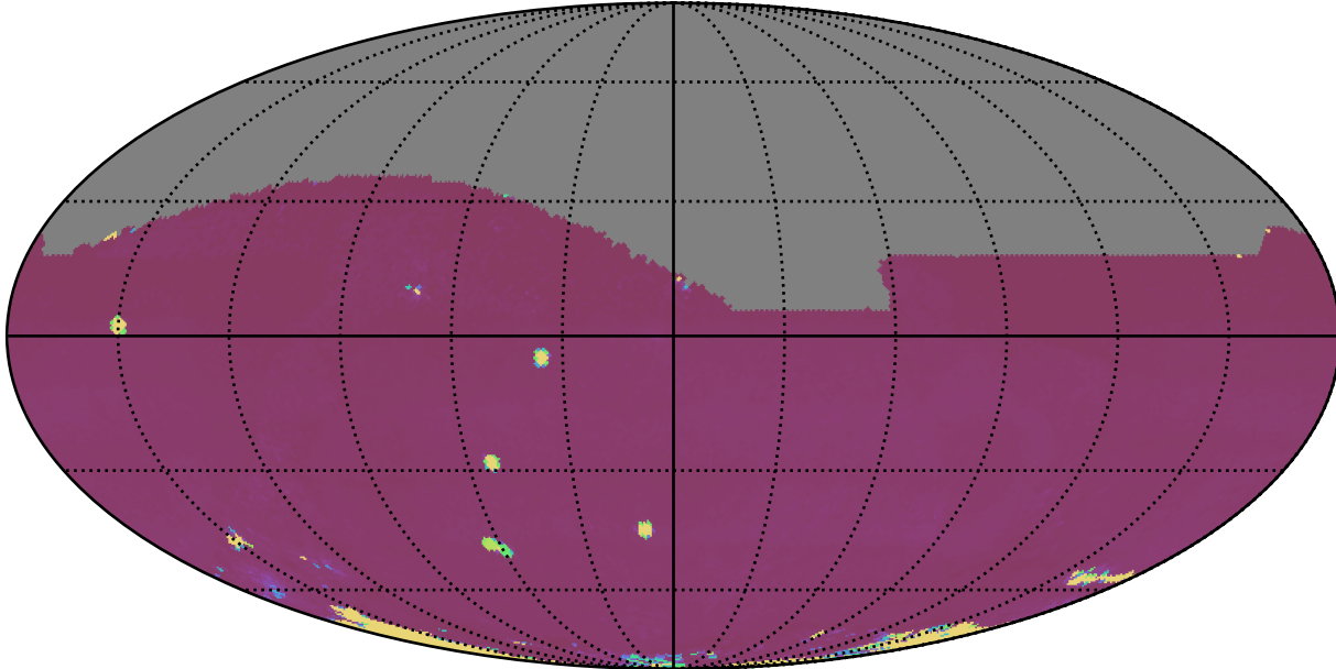
too_elab_heavy_r128_d3_ugrizy_v3.4_10yrs All sky all bands: 75th Percentile Intranight Timespan
