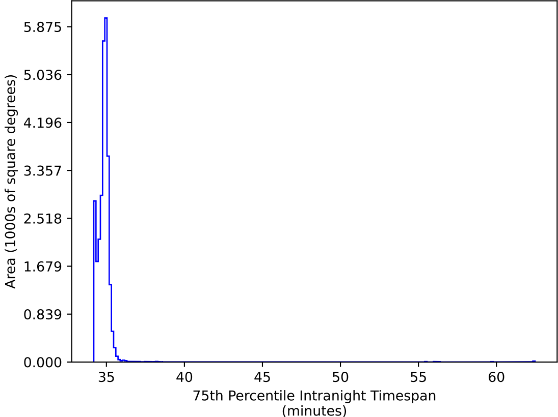
too_elab_heavy_r128_d3_ugrizy_v3.4_10yrs All sky: 75th Percentile Intranight Timespan
