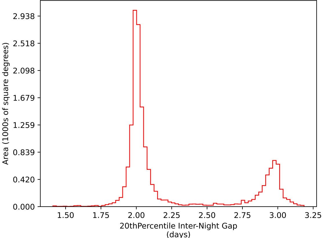
too_elab_heavy_r128_d3_ugrizy_v3.4_10yrs WFD i band: 20thPercentile Inter-Night Gap
