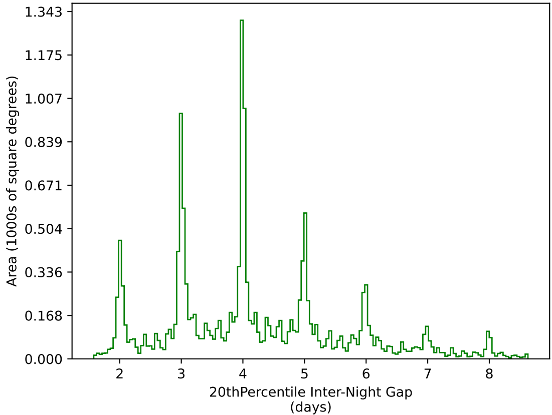
too_elab_heavy_r128_d3_ugrizy_v3.4_10yrs WFD g band: 20thPercentile Inter-Night Gap
