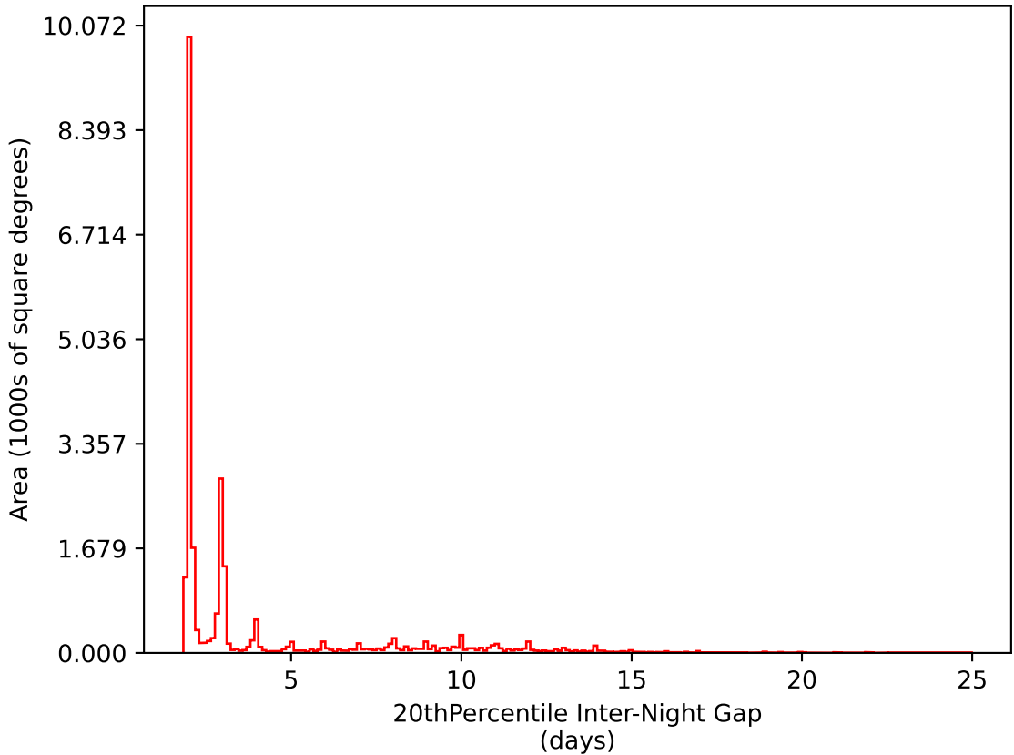
too_elab_heavy_r128_d3_ugrizy_v3.4_10yrs All sky i band: 20thPercentile Inter-Night Gap
