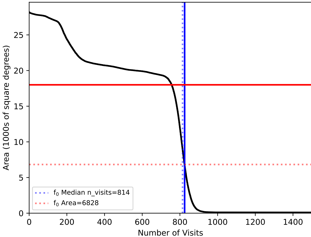
too_elab_heavy_r128_d3_ugrizy_v3.4_10yrs : f0
