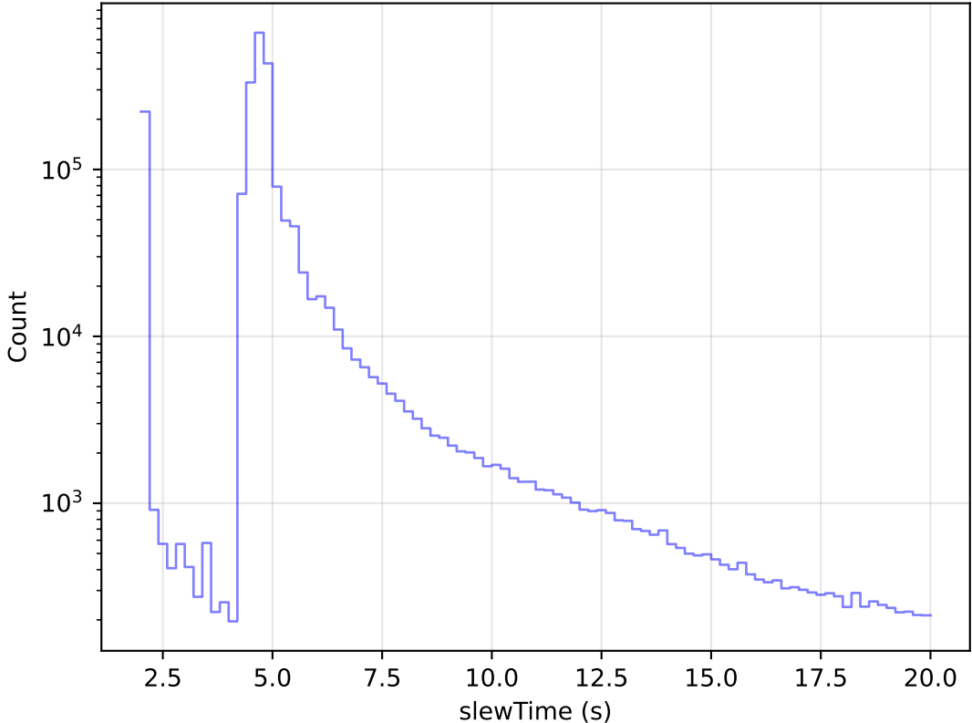
too_elab_heavy_r128_d3_ugrizy_v3.4_10yrs All visits: Zoom Slew Time Histogram
