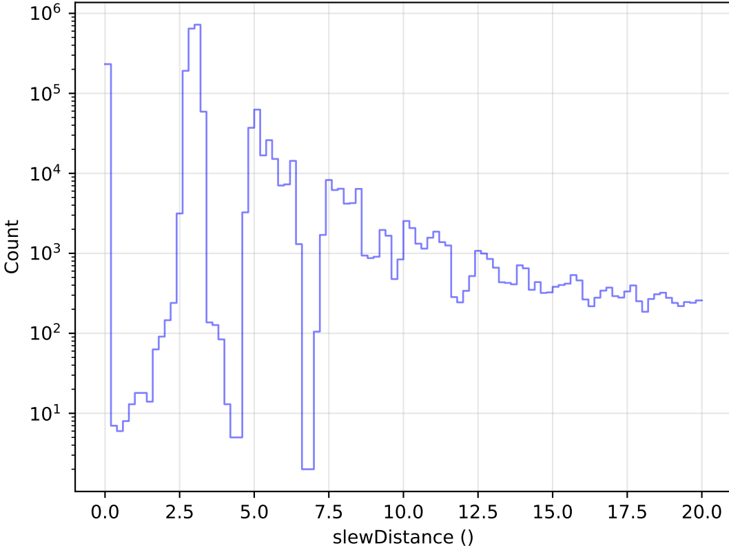
too_elab_heavy_r128_d3_ugrizy_v3.4_10yrs All visits: Zoom Slew Distance Histogram
