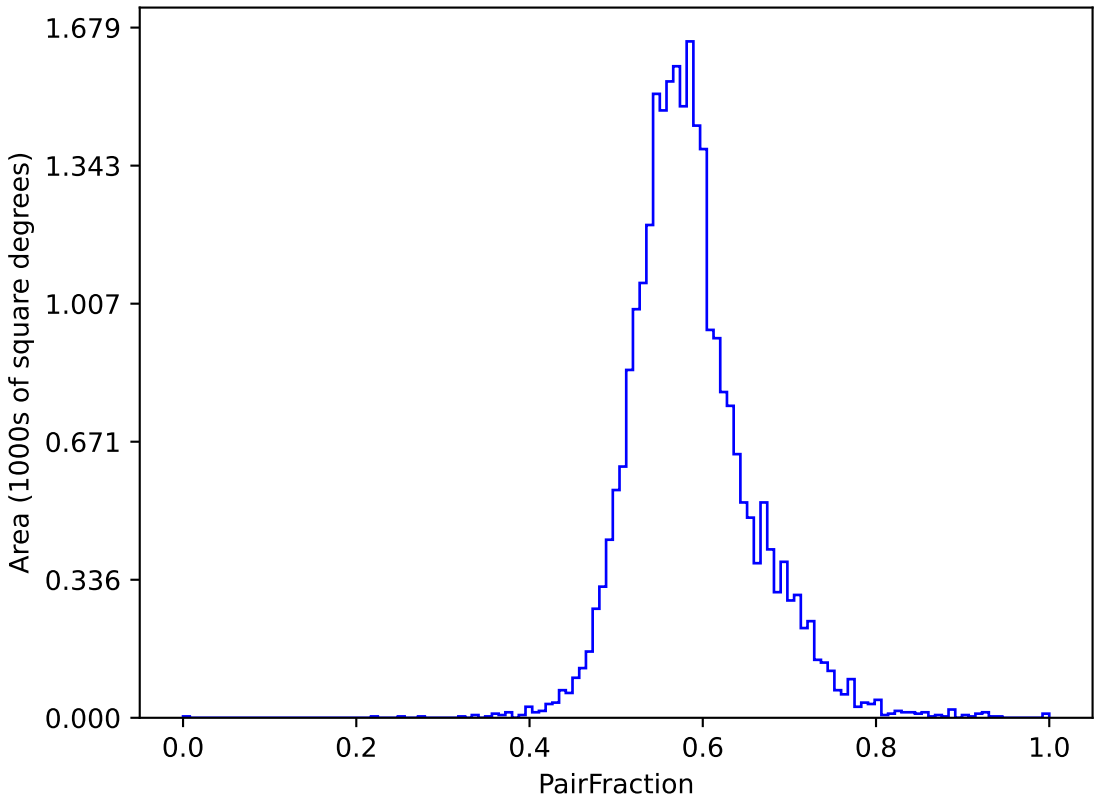
too_elab_heavy_r128_d3_ugrizy_v3.4_10yrs (g or r or i): PairFraction
