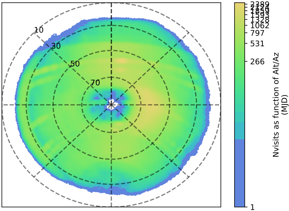
too_elab_heavy_r128_d3_ugrizy_v3.4_10yrs r: Nvisits as function of Alt/Az
