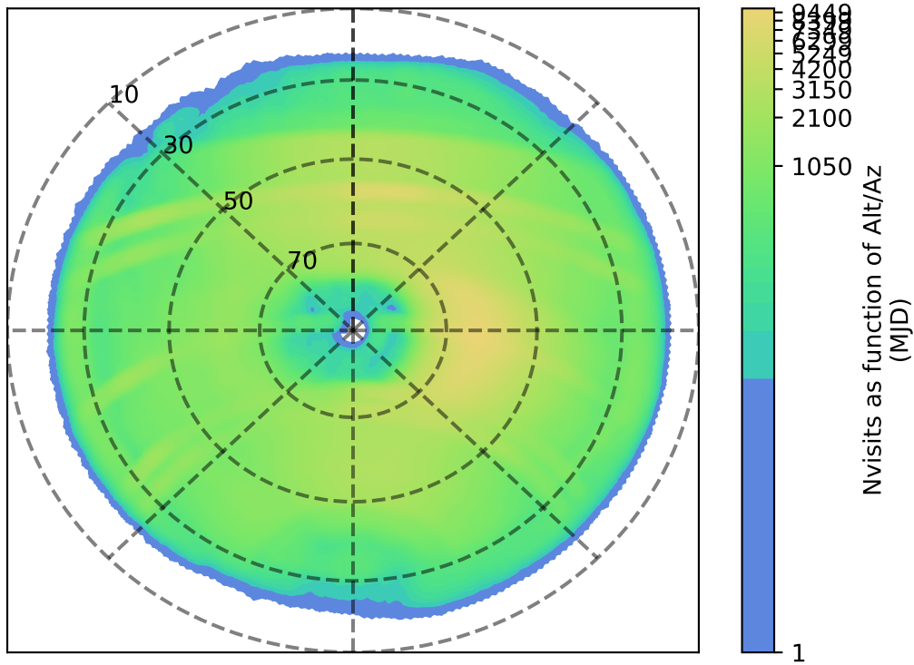
too_elab_heavy_r128_d3_ugrizy_v3.4_10yrs : Nvisits as function of Alt/Az
