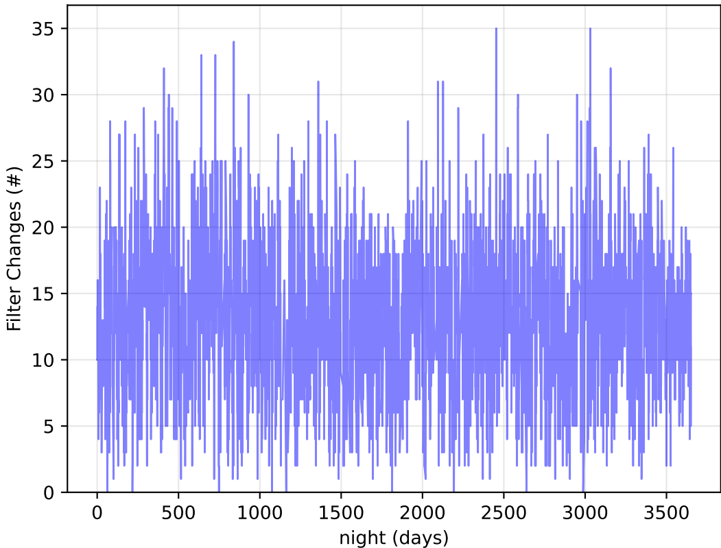
too_elab_heavy_r128_d3_ugrizy_v3.4_10yrs : Filter Changes
