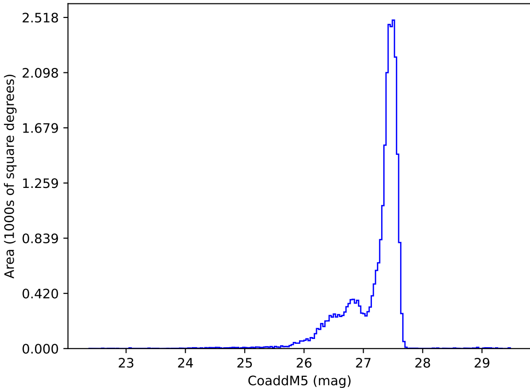
too_elab_heavy_r128_d3_ugrizy_v3.4_10yrs : CoaddM5
