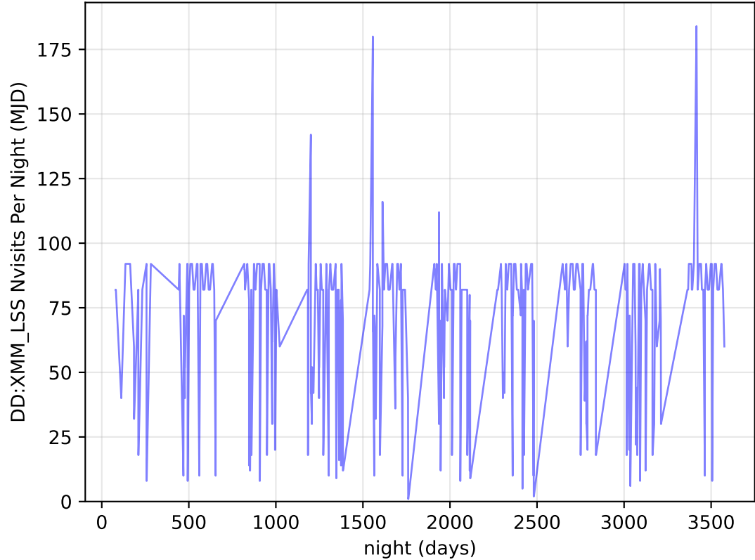
too_elab_heavy_r128_d3_ugrizy_v3.4_10yrs all bands: DD:XMM_LSS Nvisits Per Night
